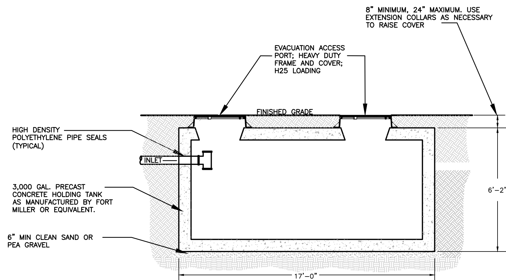
PRECAST 3,000 GALLON HOLDING TANK
