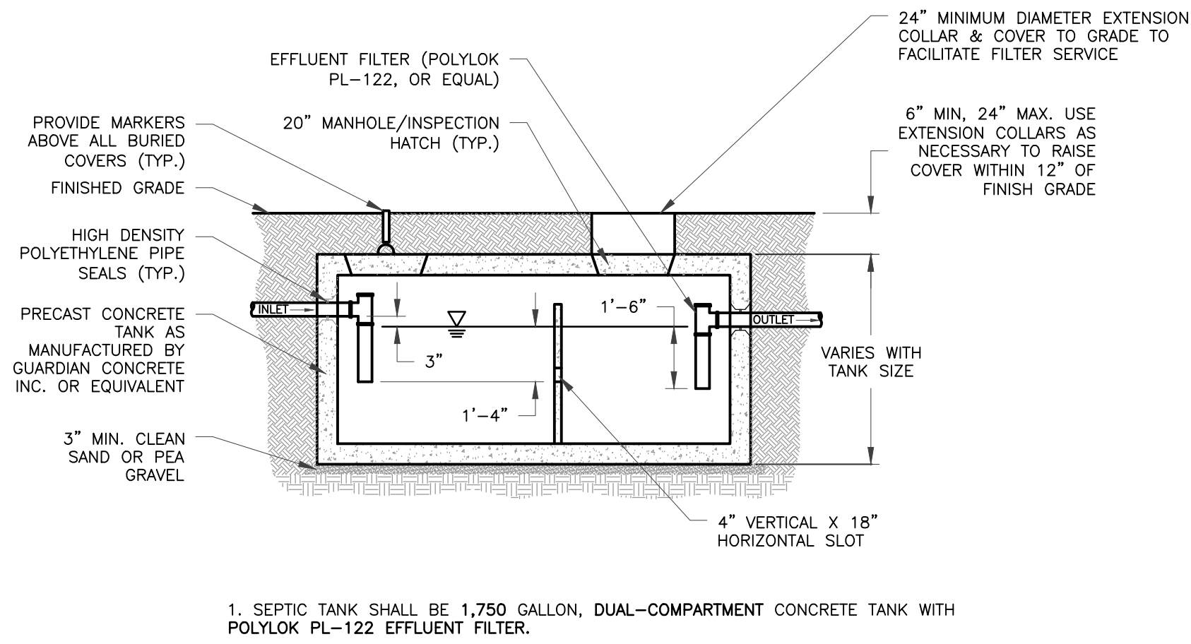
2 PRECAST SEPTIC TANK - (SEAMLESS) DUAL COMPARTMENT SCALE: NTS
