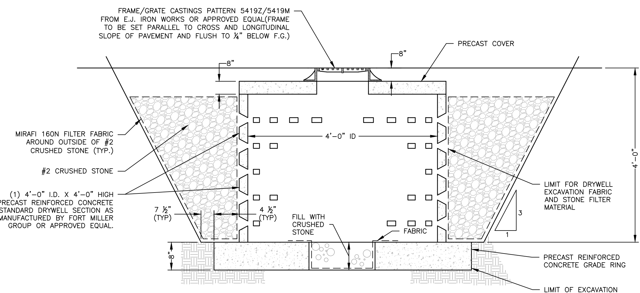
PRECAST CONCRETE DRY WELL
