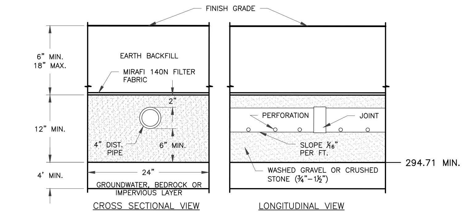
4 TYPICAL ABSORPTION TRENCH SCALE: NTS
