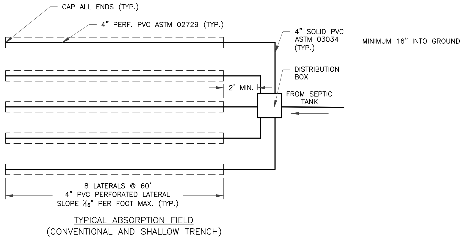
1 TYPICAL ABSORPTION FIELD SCALE: NTS
