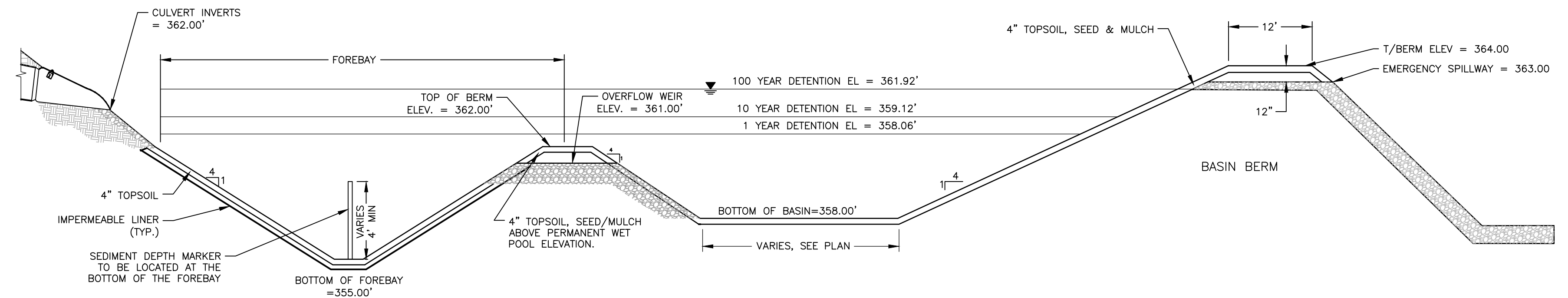
2 STORMWATER INFILTRATION BASIN 1 SCALE: NTS
