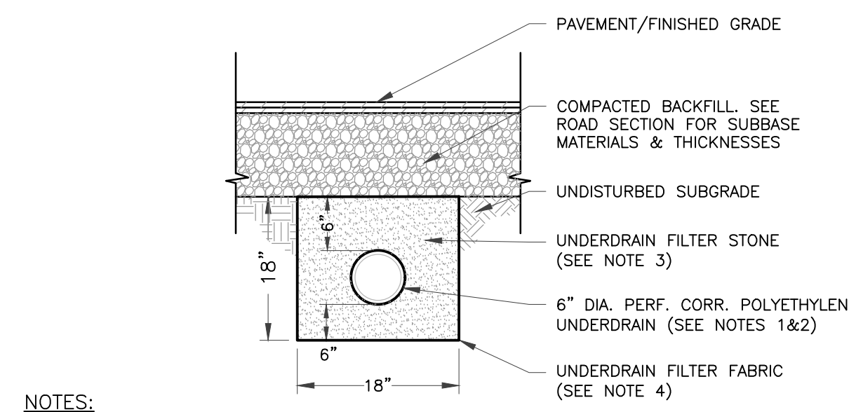
UNDERDRAIN DETAIL
