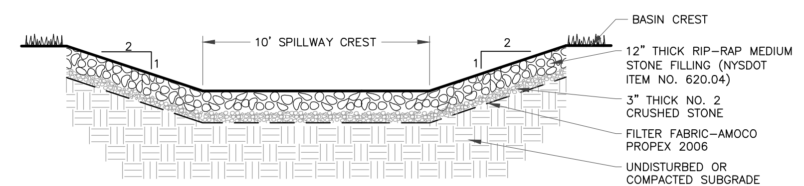
6 EMERGENCY SPILLWAY CROSS SECTION SCALE: NTS
