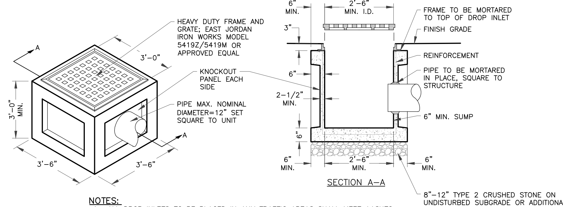
PRECAST CONCRETE MANHOLE - KNOCKOUT STRUCTURE
