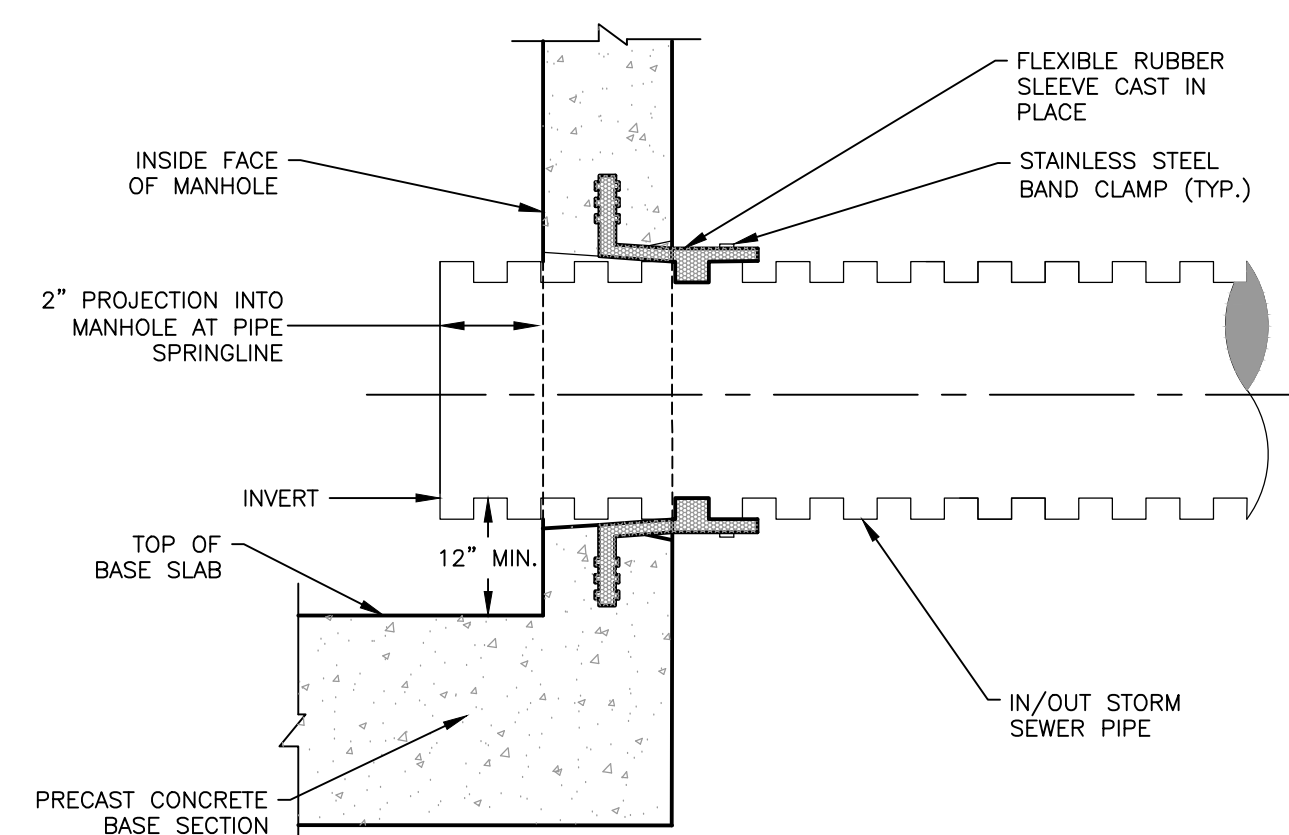
HDPE PIPE TO STRUCTURE: BOOTED JOINT
