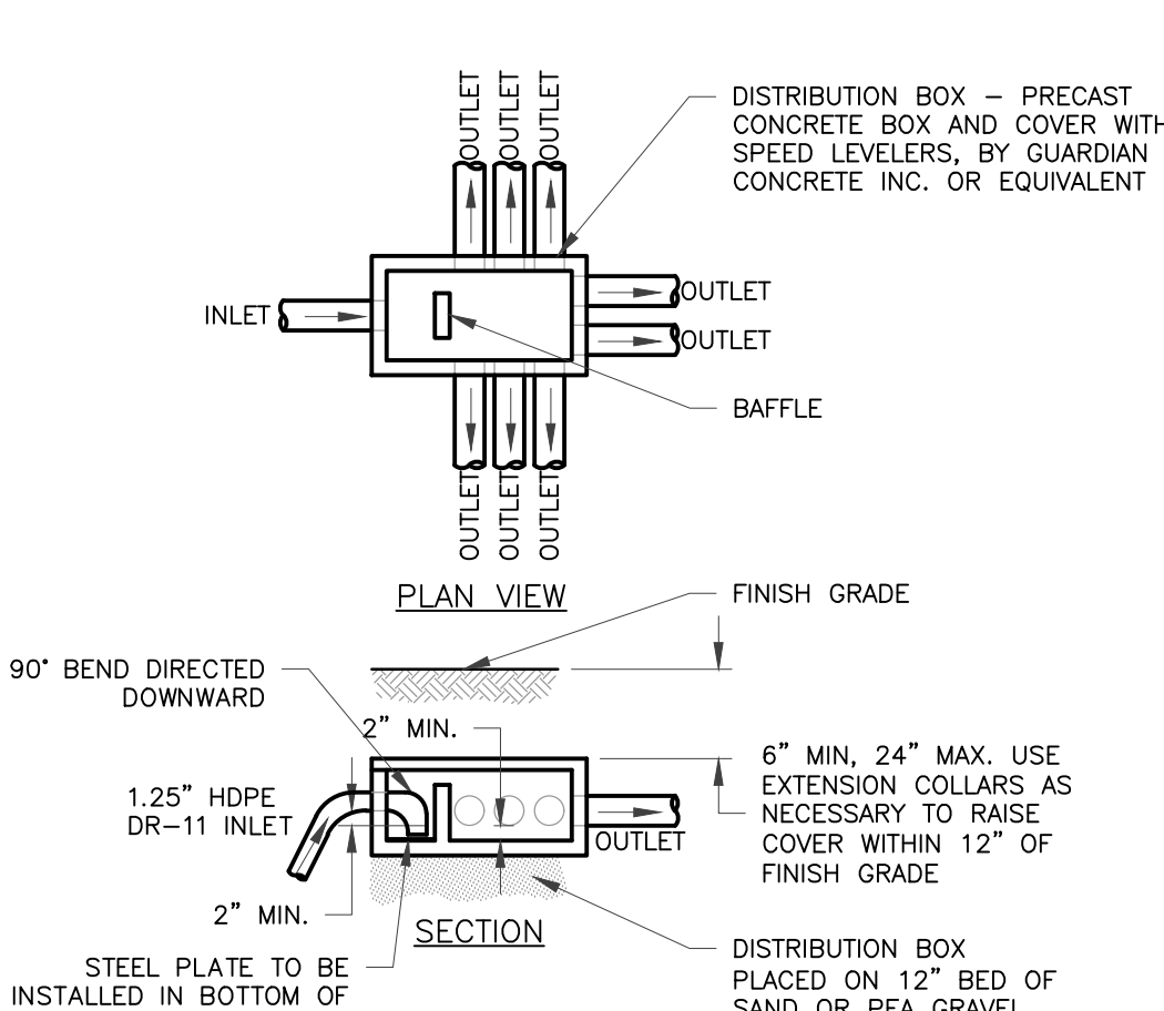
3 PRECAST DISTRIBUTION BOX SCALE: NTS
