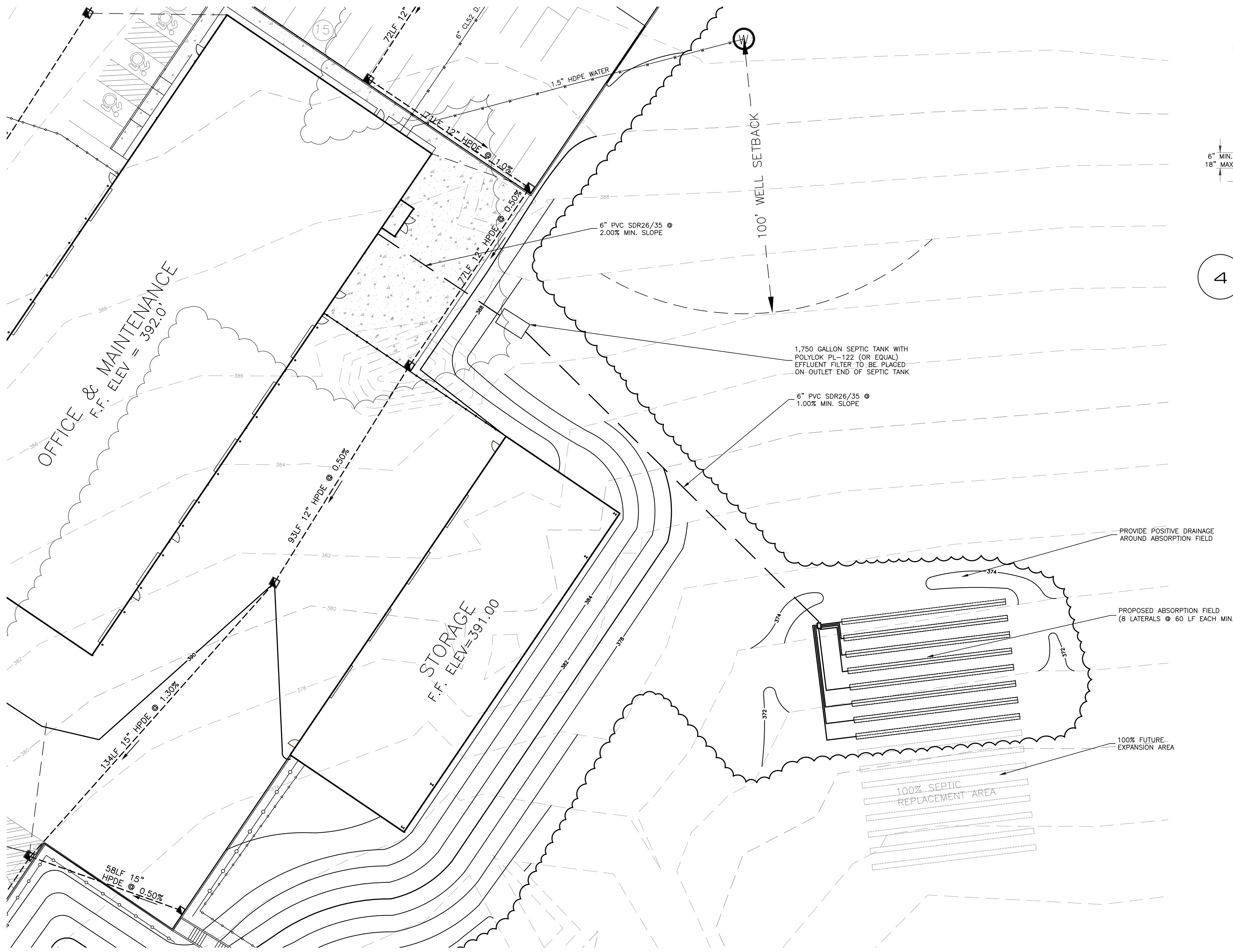
WWTS LAYOUT PLAN
